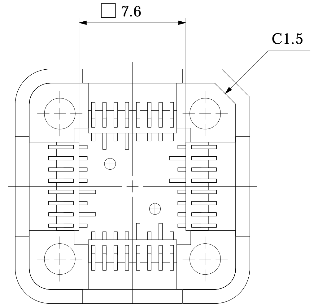
BOTTOM VIEW
