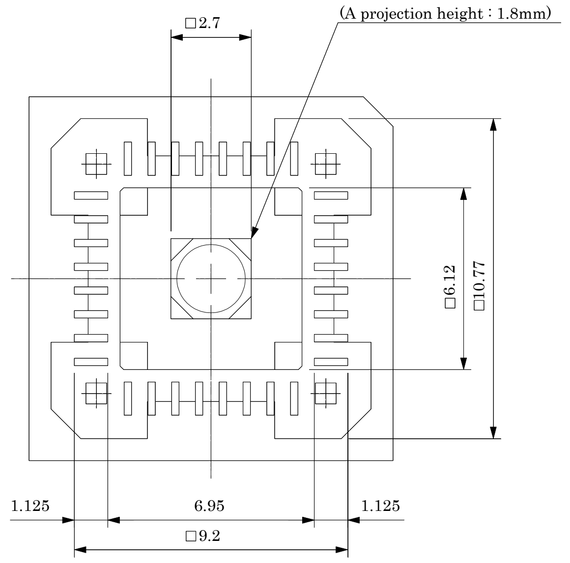
BOTTOM VIEW
