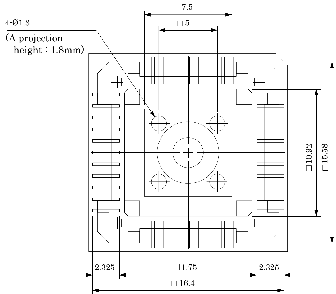
BOTTOM VIEW
