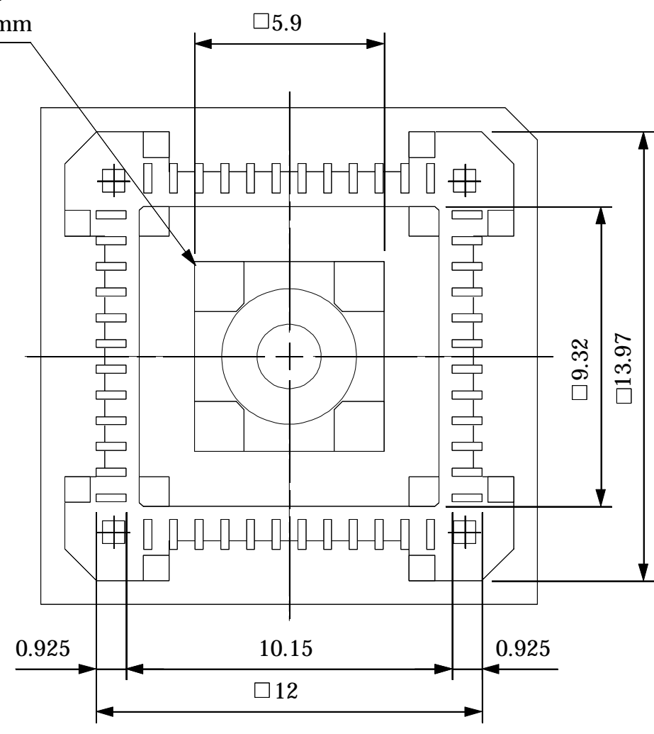
BOTTOM VIEW
