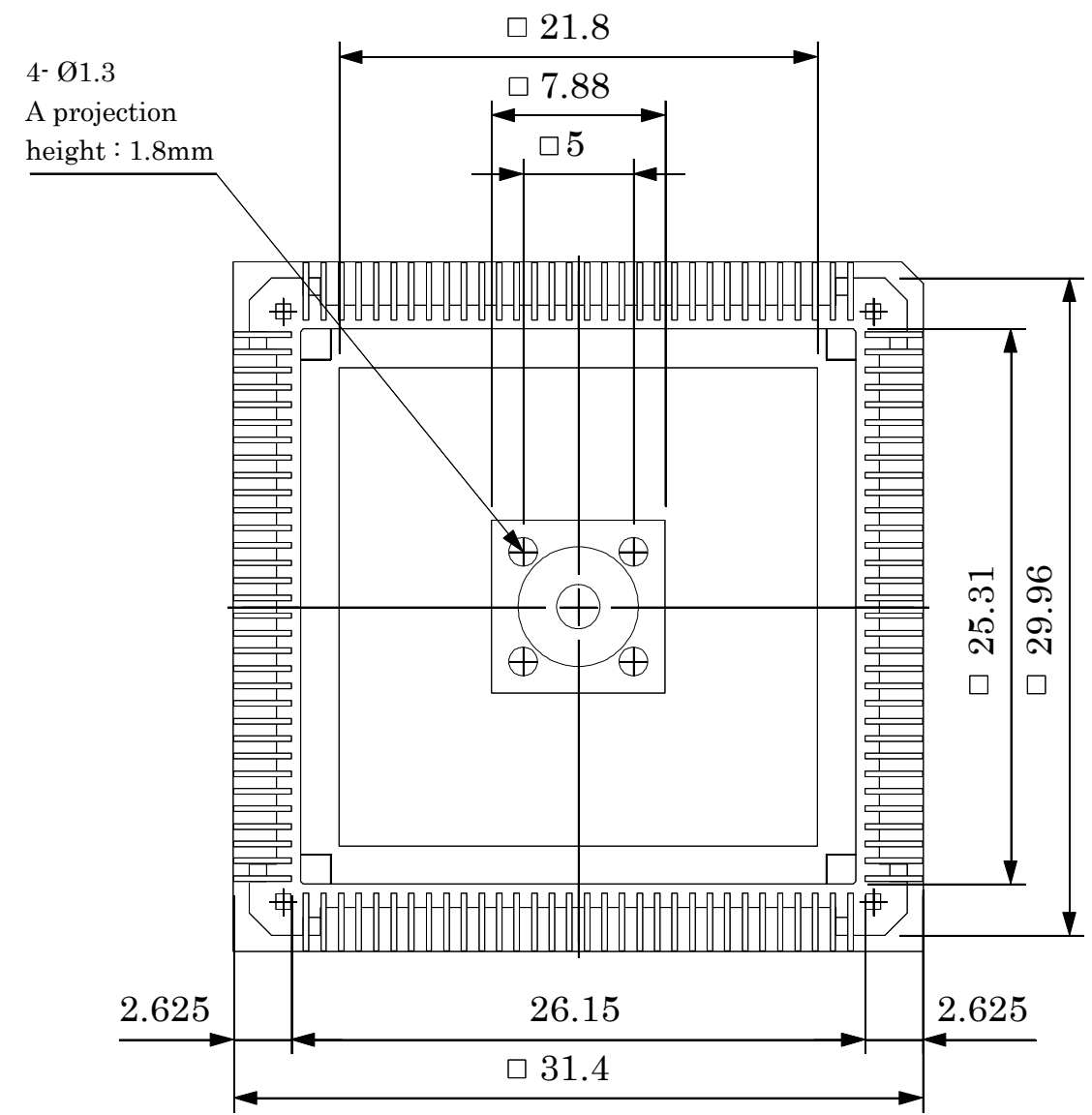
BOTTOM VIEW
