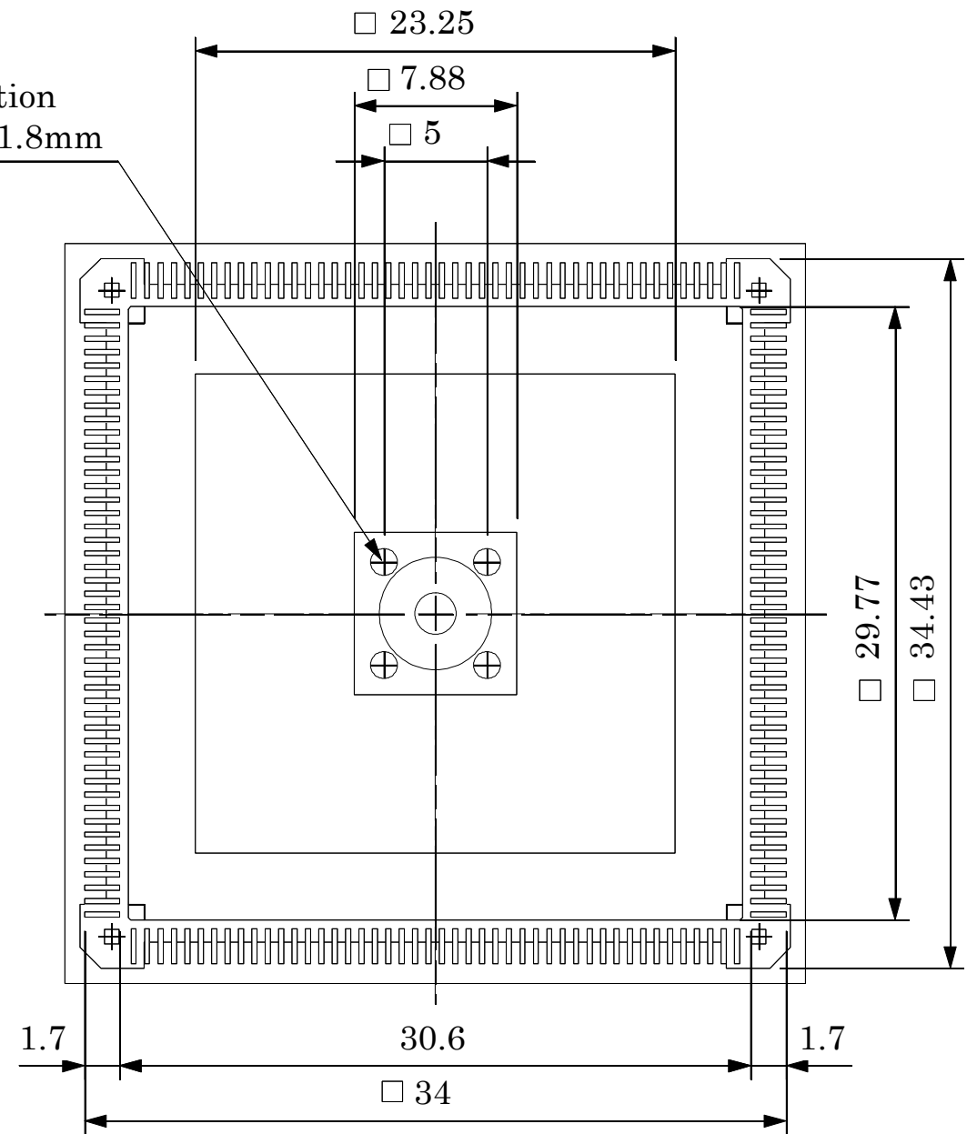
BOTTOM VIEW
