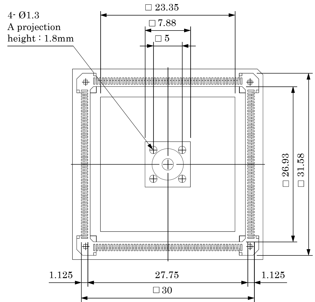
BOTTOM VIEW
